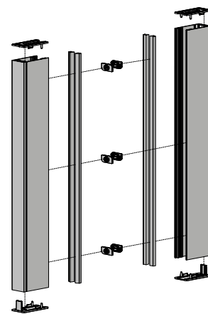
Ambience Blackout Side Guide
